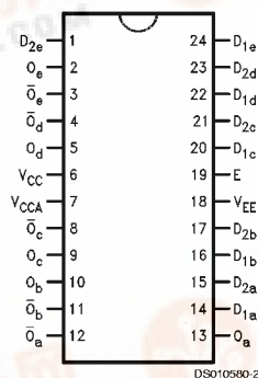
24-Pin DIP/SOIC
