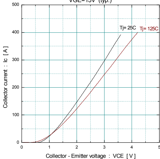
Collector current vs. Collector-Emitter voltage VGE = 15V (typ.)
