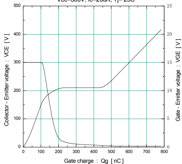
Dynamic Gate charge (typ.) Vcc = 300V, Ic = 200A, T j = 25°C
