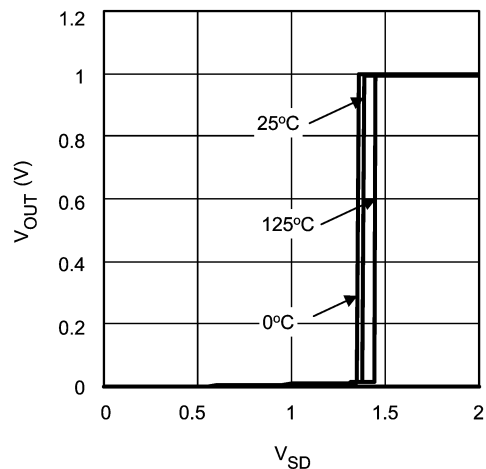
Turn-On Characteristics
