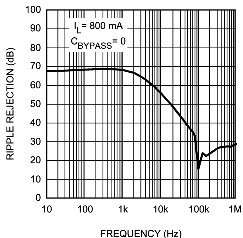
Ripple Rejection
