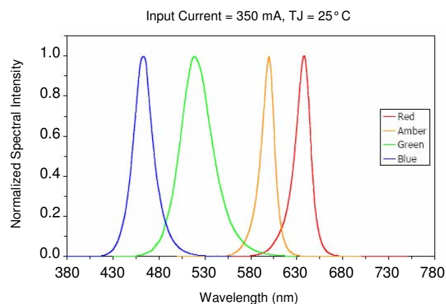
Wavelength Characteristics
