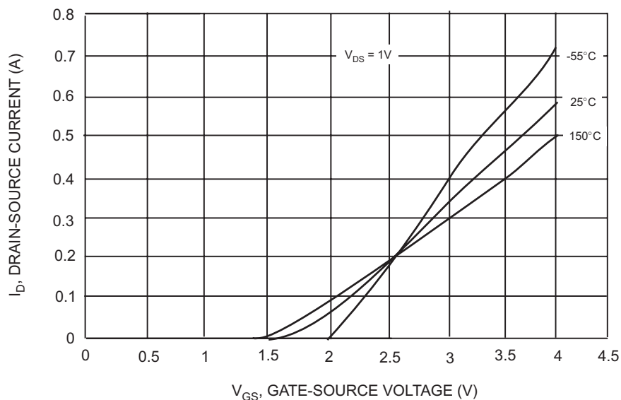
Fig. 2 Transfer Characteristics
