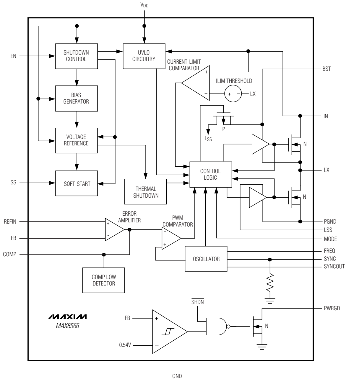
Figure 1. Functional Diagram
