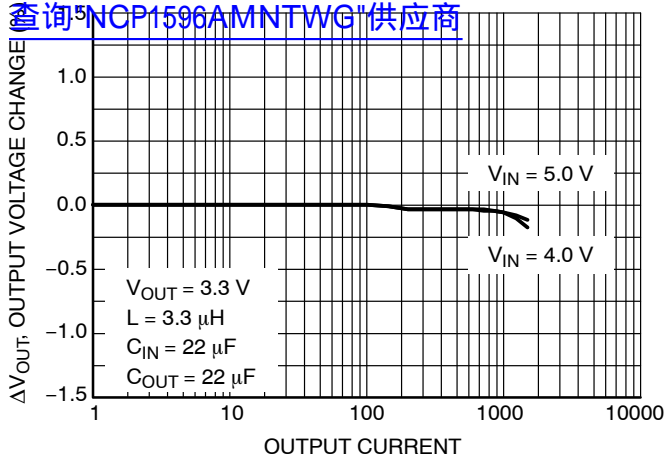
Figure 11. Output Voltage Change vs. Output Current
