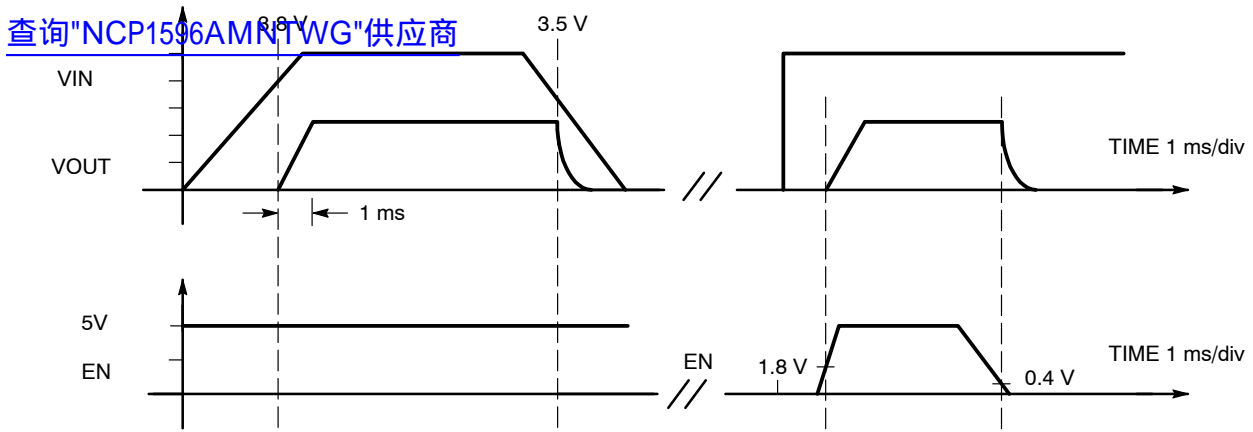
Figure 3. Timing Diagram
