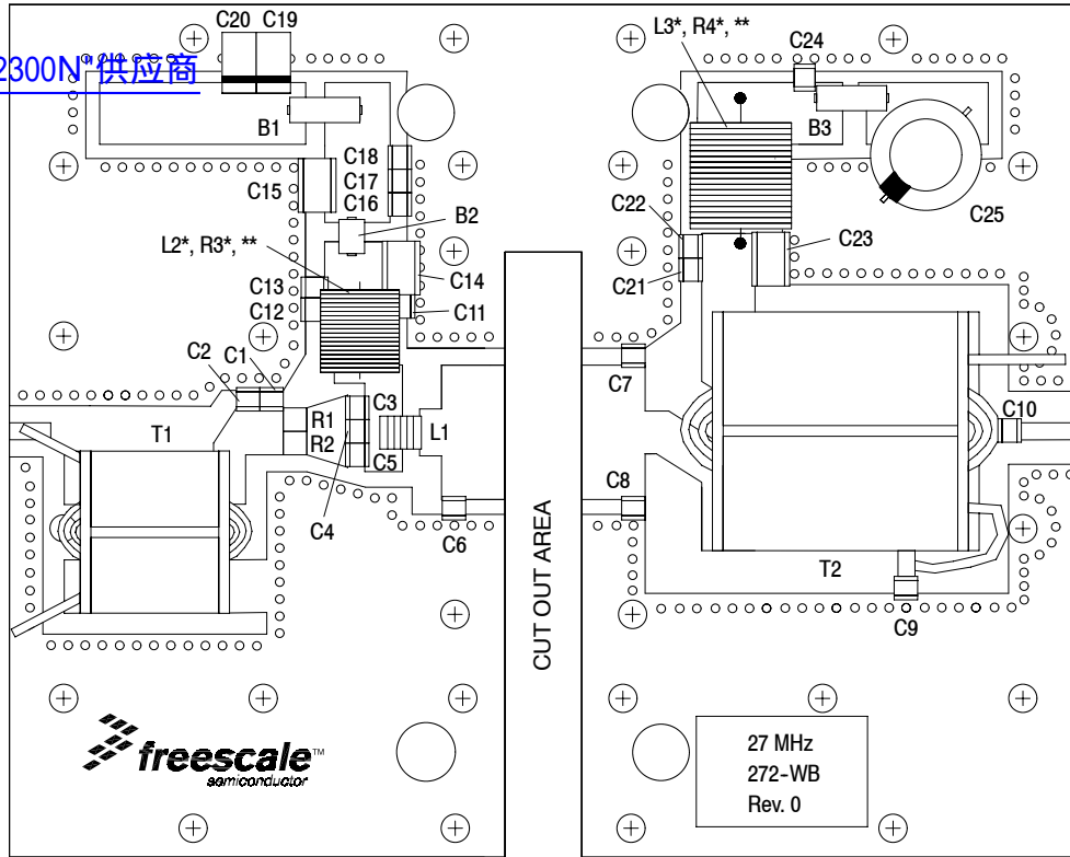
Figure 16. MRF6V2300NR1 (NBR1) Test Circuit Component Layout — 27 MHz
