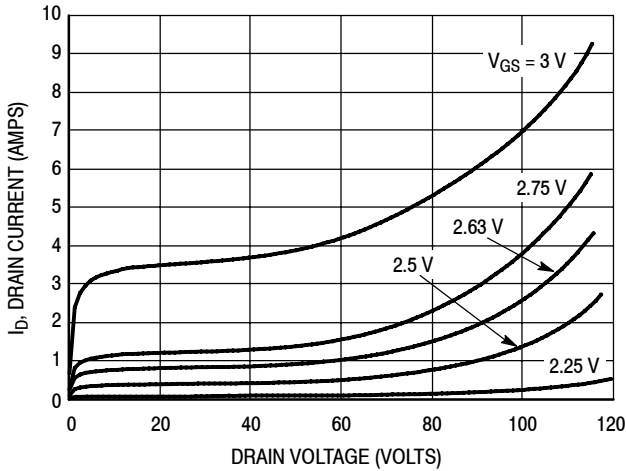
Figure 6. DC Drain Current versus Drain Voltage
