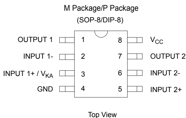
Figure 2. Pin Configuration of CP103
