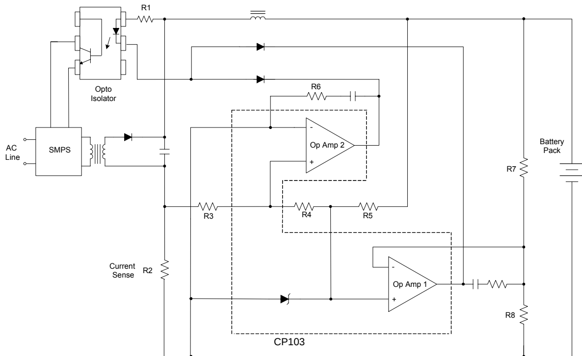
Figure 8. Application of CP103 in a Constant Current and Constant Voltage Charger
