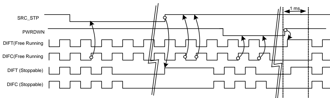
Figure 8. SRC_STP = Tri-state, PWRDWN = Tri-state, OE_INV = 0
