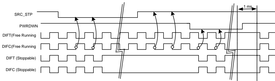
Figure 6. SRC_STP = Driven, PWRDWN = Driven, OE_INV = 0
