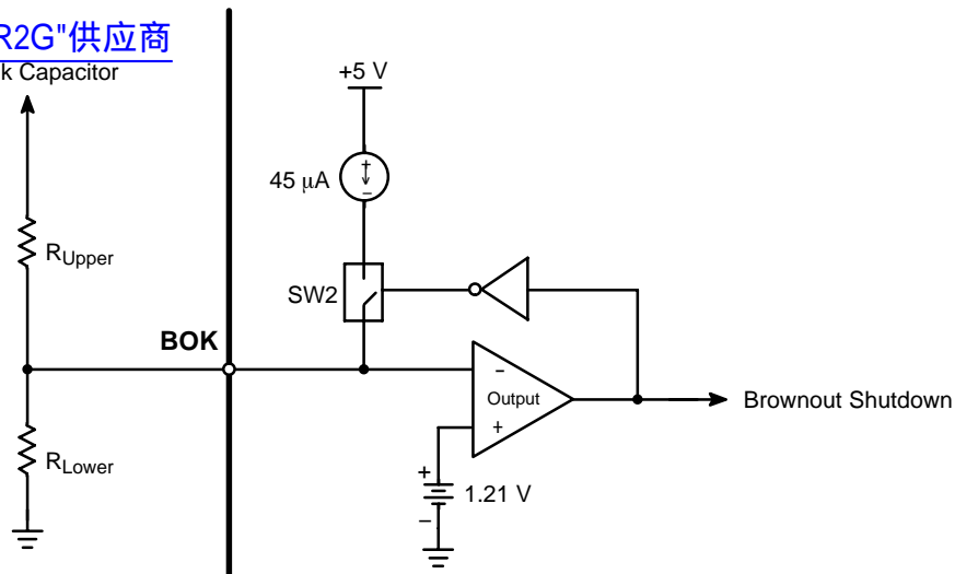
Figure 39. Brownout Detect Block Diagram
