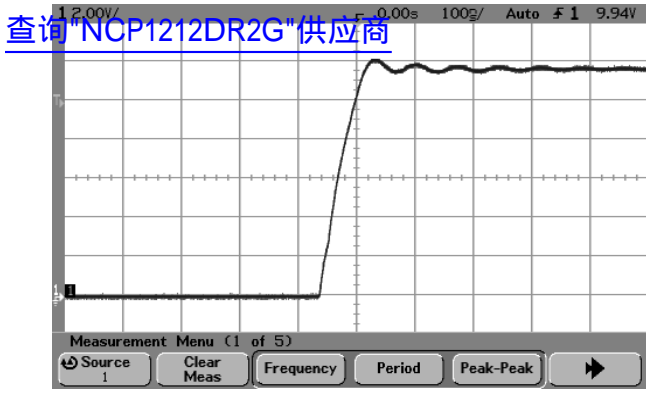
Figure 27. Rise Time of Gate Drive Waveform ( C_L = 1 \text{ nF} )
