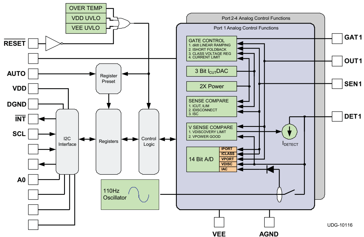
Figure 23. Block Diagram
