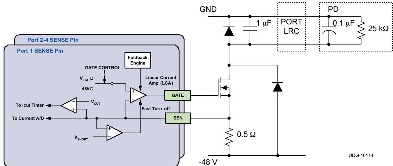
Figure 22. Port Current Sense Circuitry
