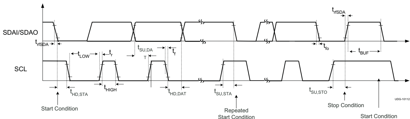
Figure 24. I²C Timings
