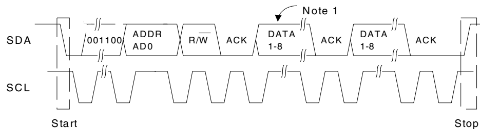
Figure 18. Control Port Timing, I 2 C Mode
