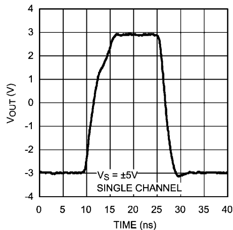
6 V pp Pulse Response
