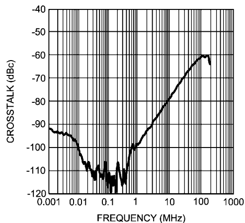
2 V pp Off Isolation
