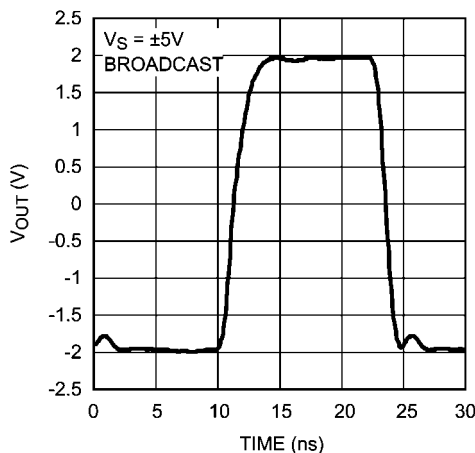
4 V PP Pulse Response Broadcast
