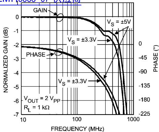
Frequency Response 1 k \Omega Load 查询"LMH6583 07"供应商
