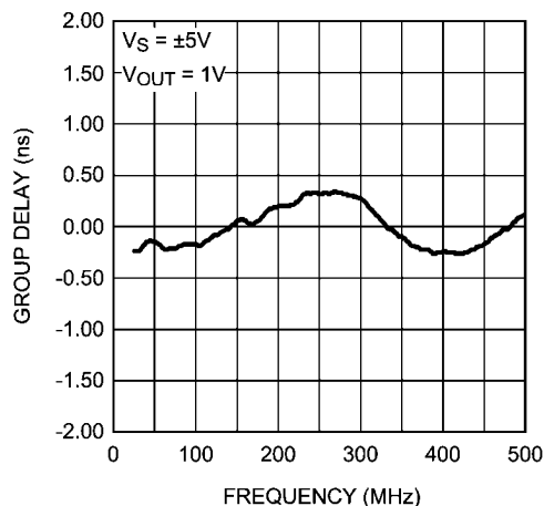
Group Delay
