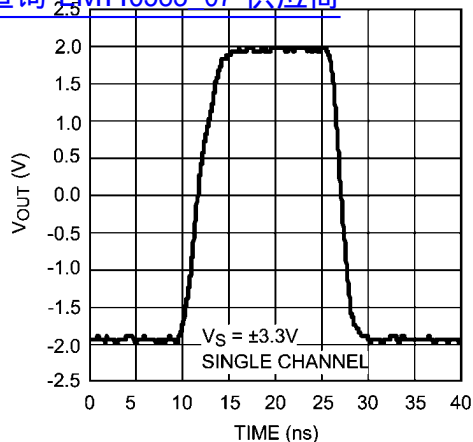
4 V pp Pulse Response 查询"LMH6583 07"供应商
