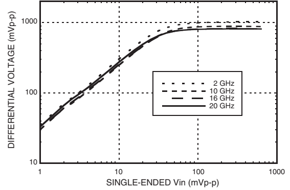
Differential Output vs. Vinut & Frequency [1] [2]
