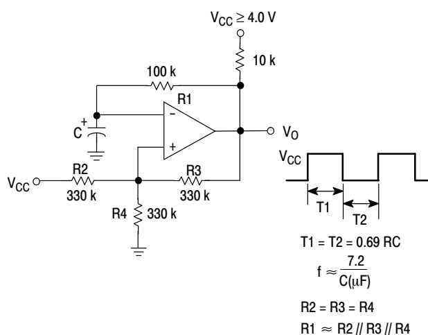
Figure 8. Squarewave Oscillator
