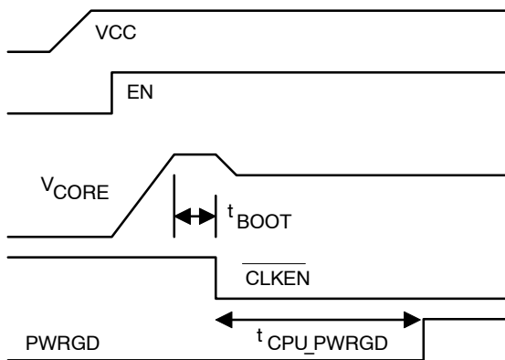
Figure 22. Powerup Sequence
