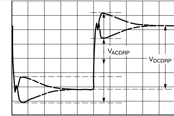
Figure 28. AC Load Line Waveform
