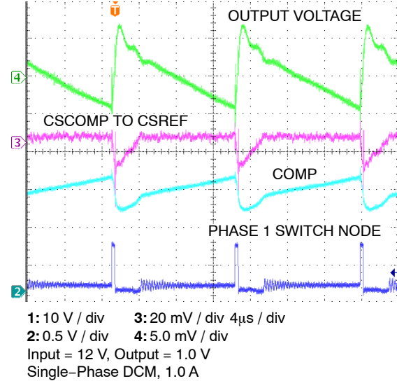
Figure 14. Switching Waveforms
