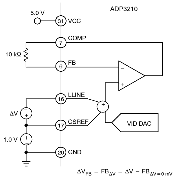
Figure 4. Positioning Accuracy
