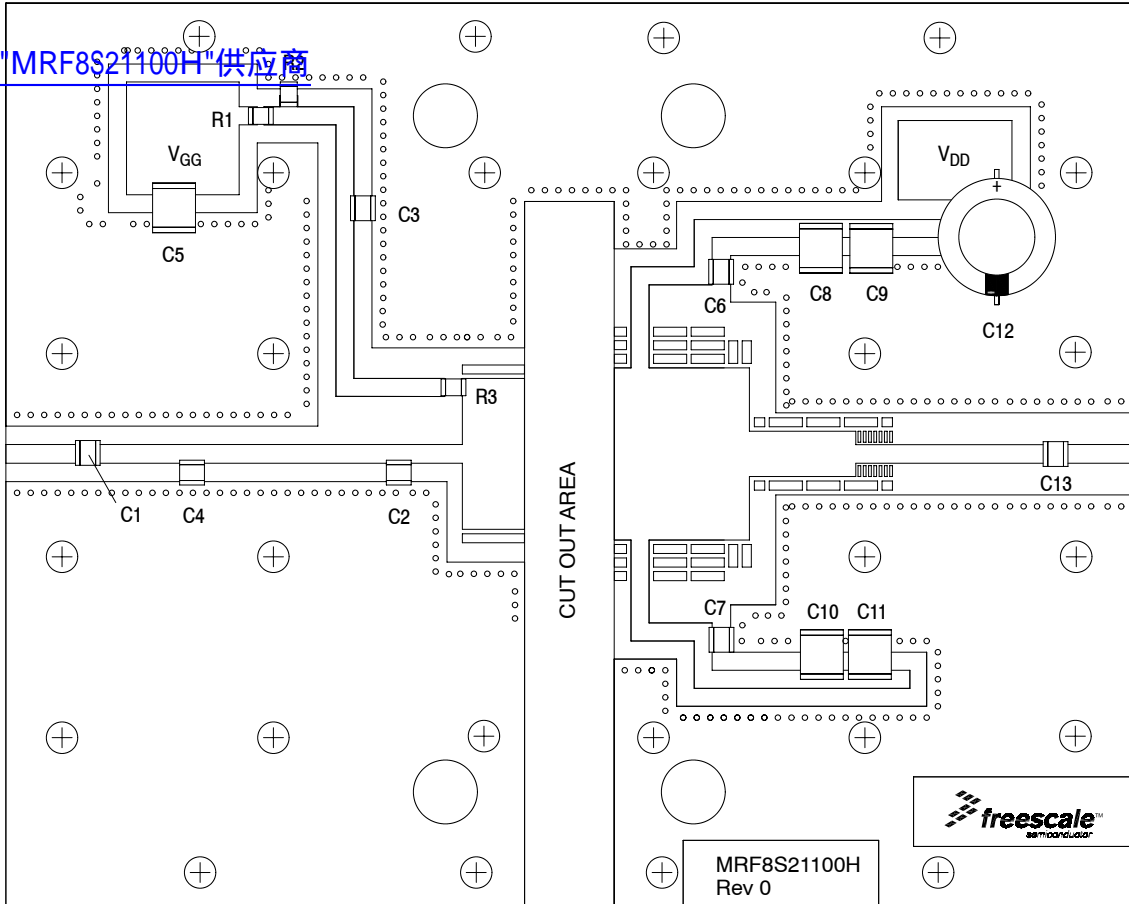
Figure 1. MRF8S21100HR3(HSR3) Test Circuit Component Layout
