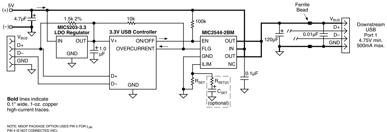
Figure 4. USB Host Application
