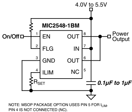
Figure 3. Supply Bypassing
