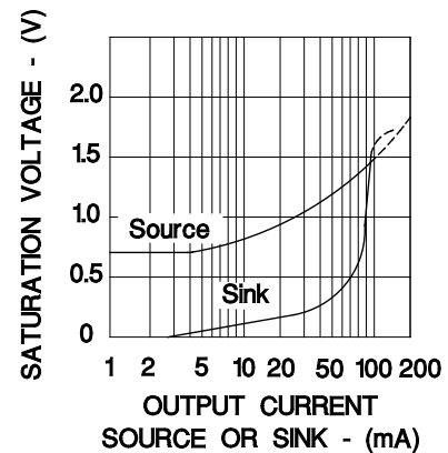
Output Driver Saturation Voltage
