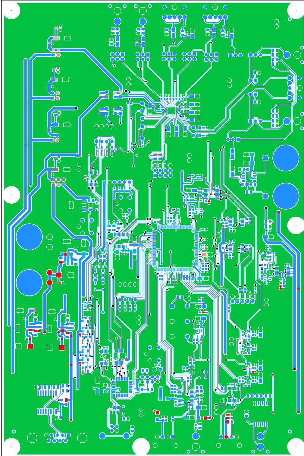
Figure 35. Top-Side Layer
