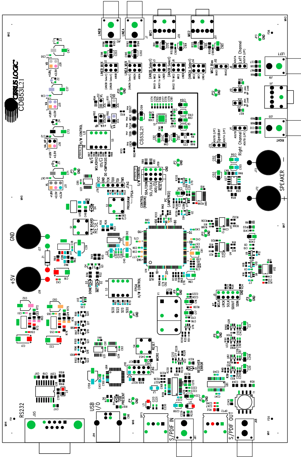
Figure 34. Silk Screen
