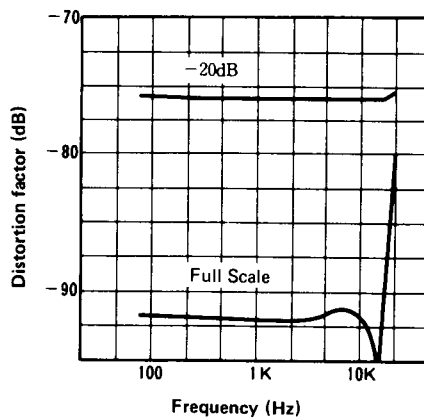
Distortion factor
