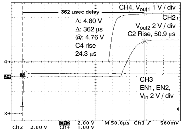
Figure 15. Typical Turn-on Delay for 3.3 V out 1 mA, 5.0 V out 200 mA Output with Simultaneous V in and Enable
