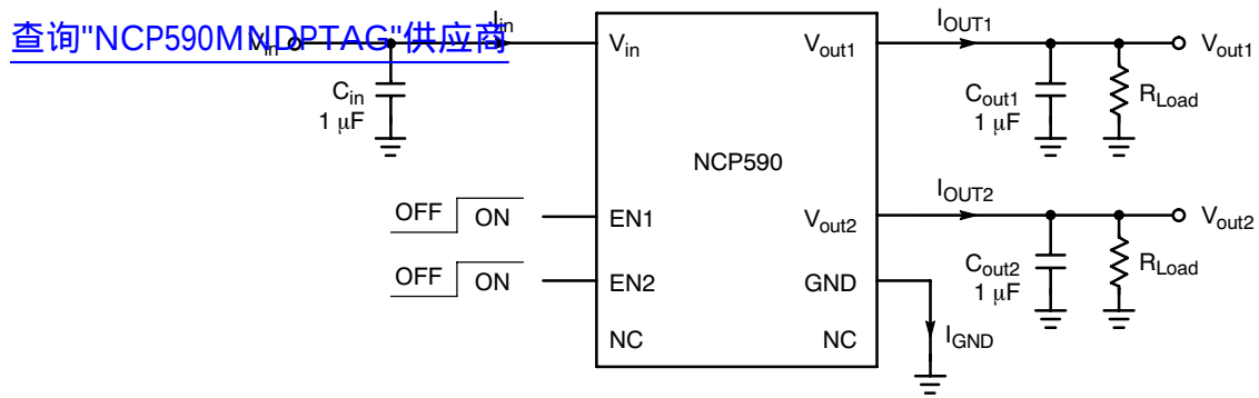
Figure 3. Measuring Circuit
