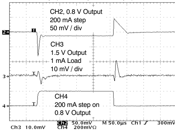
Figure 14. Load Transient on 0.8 V out and Effect on 1.5 V out for 200 mA Step
