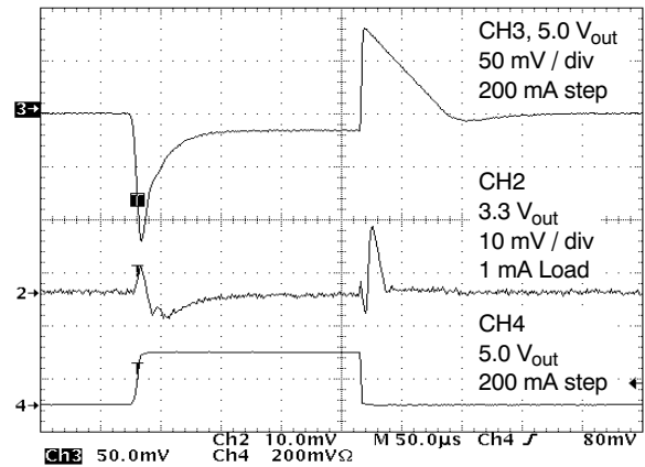
Figure 13. Load Transient on 5.0 V out and Effect on 3.3 V out for 200 mA Step
