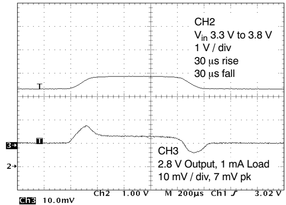
Figure 11. 2.8 V out vs. Line Transient
