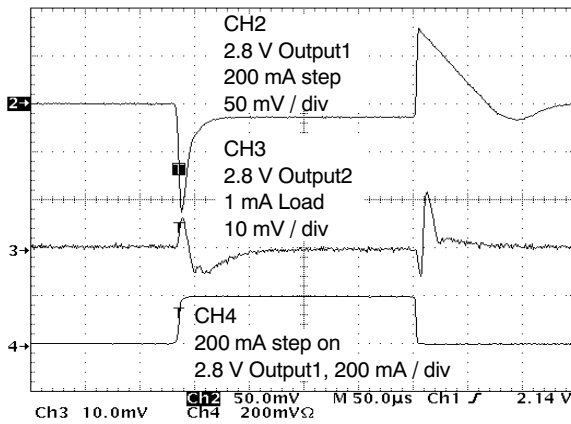
Figure 12. Load Transient on 2.8 V out and Effect on 2.8 V out for 200 mA Step
