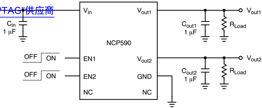
Figure 1. Typical Application
