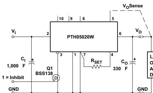
Figure 13. Inhibit Control Circuit
