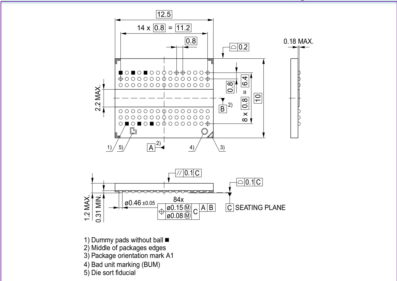
FIGURE 9 Package Outline PG-TFBGA-84
