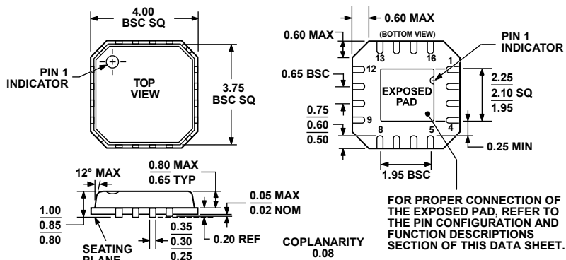
COMPLIANT TO JEDEC STANDARDS MO-220-VGGC Figure 43. 16-Lead Lead Frame Chip Scale Package [LFCSP_VQ] 4 mm x 4 mm Body, Very Thin Quad (CP-16-4) Dimensions shown in millimeters
