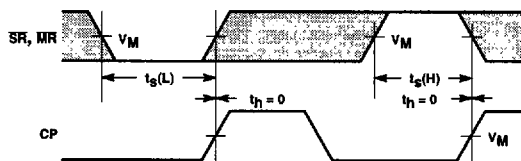
Waveform 6. Synchronous Reset Setup, Pulse Width and Hold Times (54F163A)
