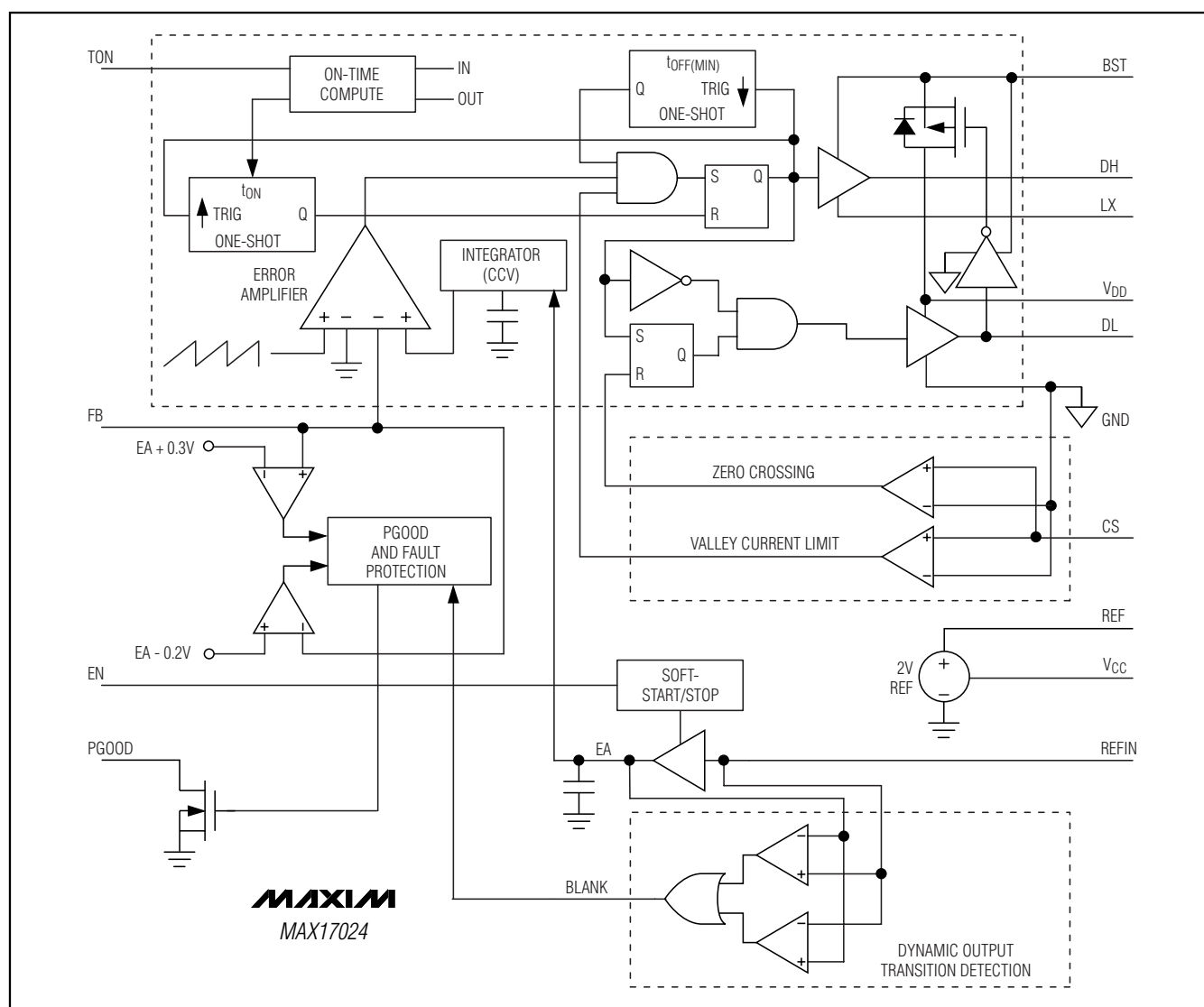
Figure 2. MAX17024 Functional Block Diagram
