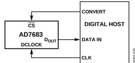
Figure 25. Connection Diagram
