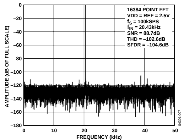
Figure 12. FFT Plot
