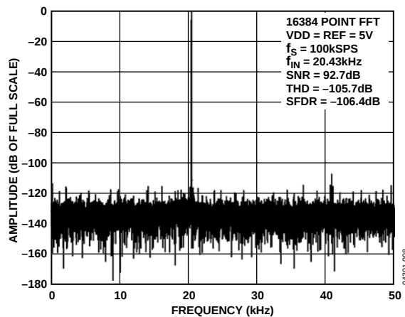
Figure 9. FFT Plot
