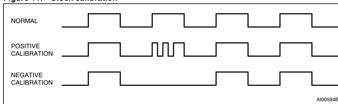
Figure 11. Clock calibration
