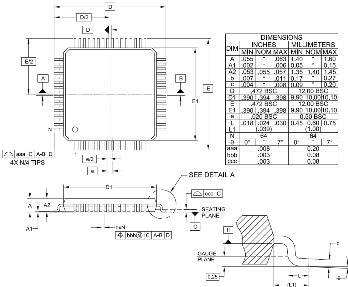
Figure 6 LQFP Package
