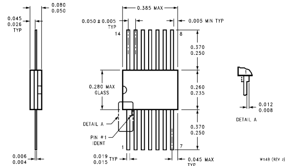
14-Lead Ceramic Flat Package (W) Order Number 54LS08FMQB or DM54LS08W NS Package Number W14B
