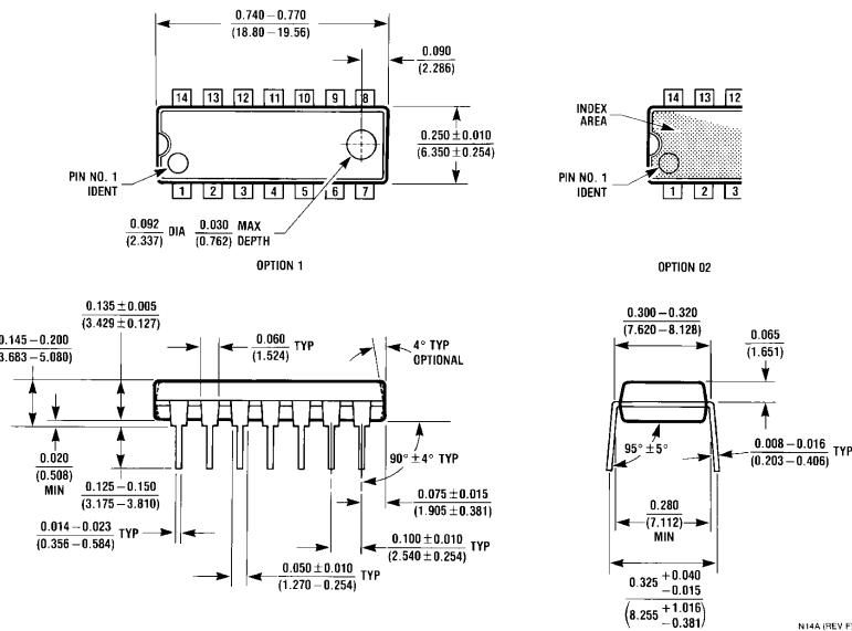
14-Lead Molded Dual-In-Line Package (N) Order Number DM74LS08N NS Package Number N14A
