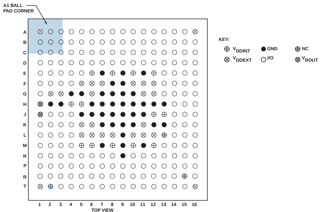
Figure 46. 256-Ball CSP_BGA Ball Configuration (Top View)
