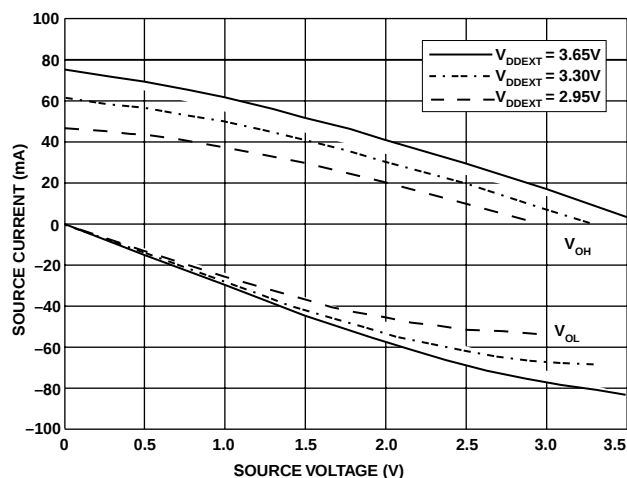
Figure 32. Drive Current C (High V_{DDEXT} )
