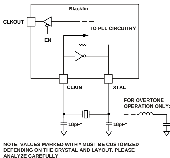
Figure 5. External Crystal Connections
