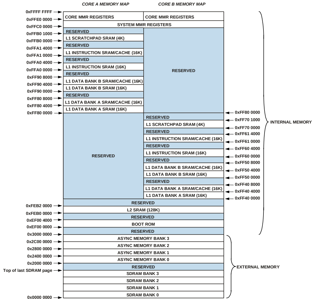
Figure 3. Memory Map
