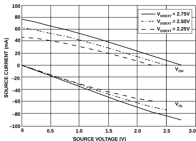
Figure 33. Drive Current D (Low V_{DDEXT} )
