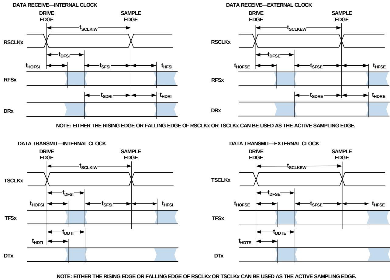
Figure 19. Serial Ports
