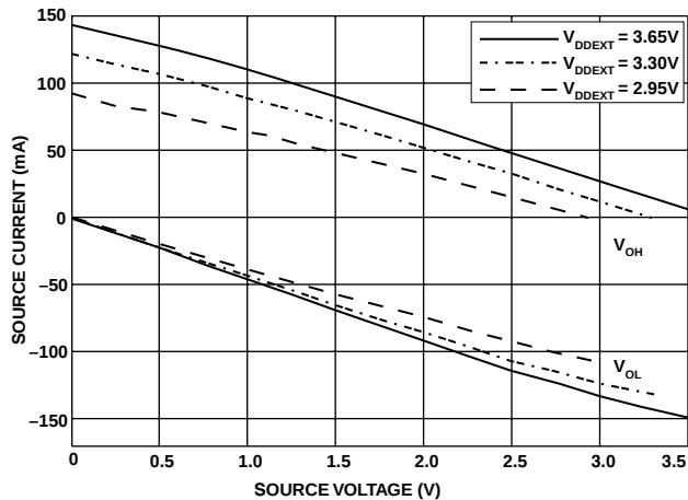
Figure 28. Drive Current A (High V_{DDEXT} )
