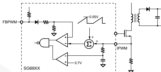
Figure 8. Slope Compensation
