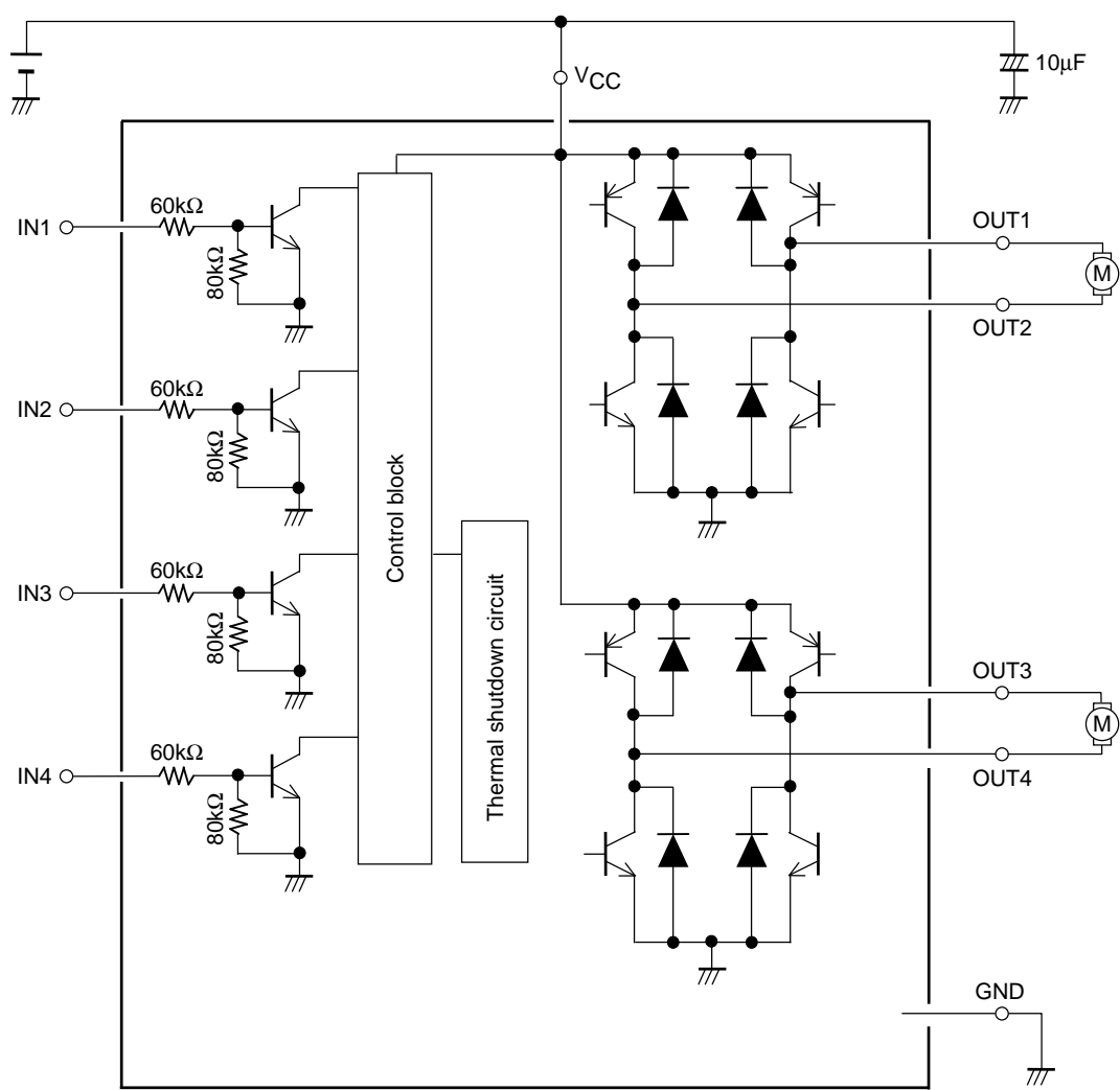
Block Diagram
