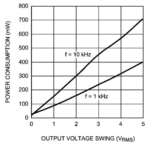
Power Consumption vs Output Voltage Swing V_{DD} = 3.6V , THD+N ≤ 1%
