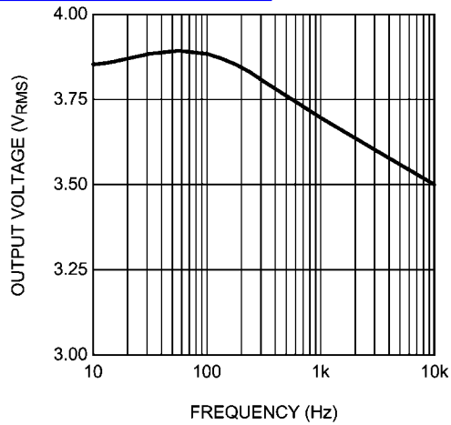
Output Voltage vs Frequency V_{DD} = 2.7V , THD+N = 1%
