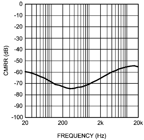
CMRR vs Frequency V_{DD} = 7V , Input referred
