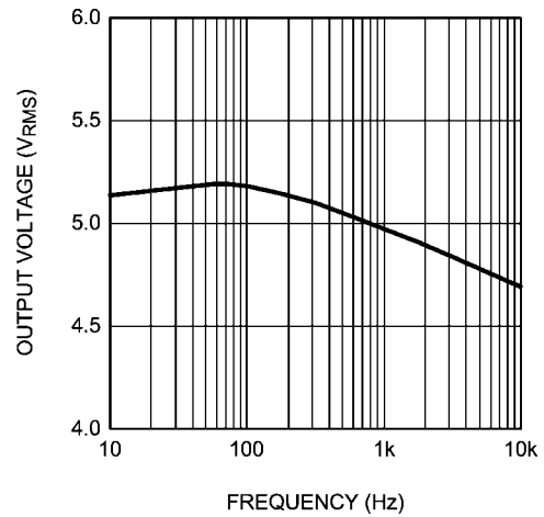
Output Voltage vs Frequency V_{DD} = 3.6V , THD+N = 1%
