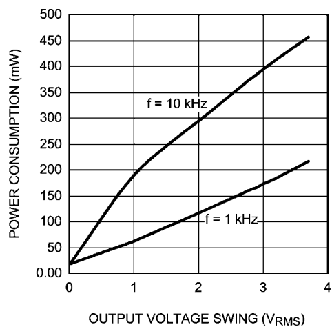
Power Consumption vs Output Voltage Swing V_{DD} = 2.7V , THD+N ≤ 1%
