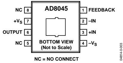
Figure 5. SOIC Pin Configuration
