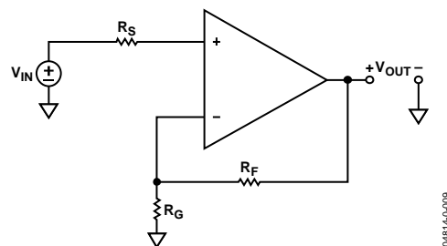
Figure 64. Noninverting Configuration
