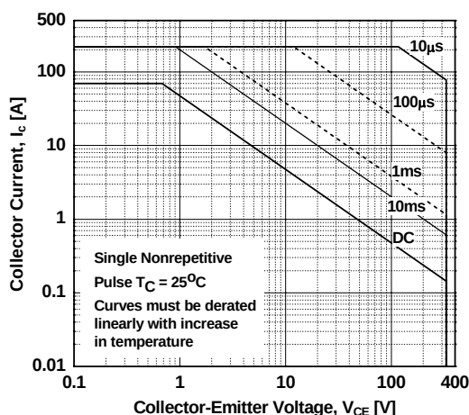
Figure 10. SOA Characteristics
