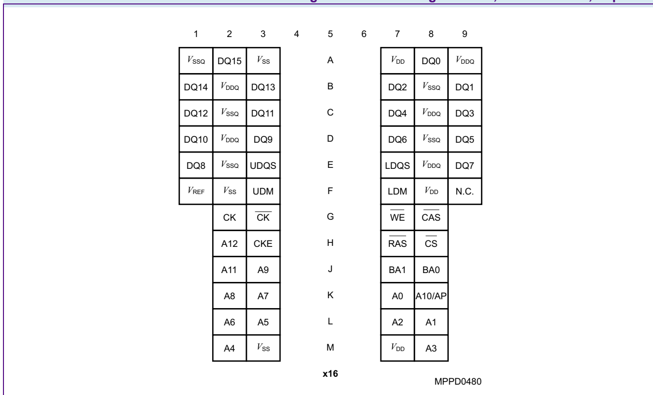
FIGURE 3 Pin Configuration for x16 Organization, PG-TFBGA-60, Top View
