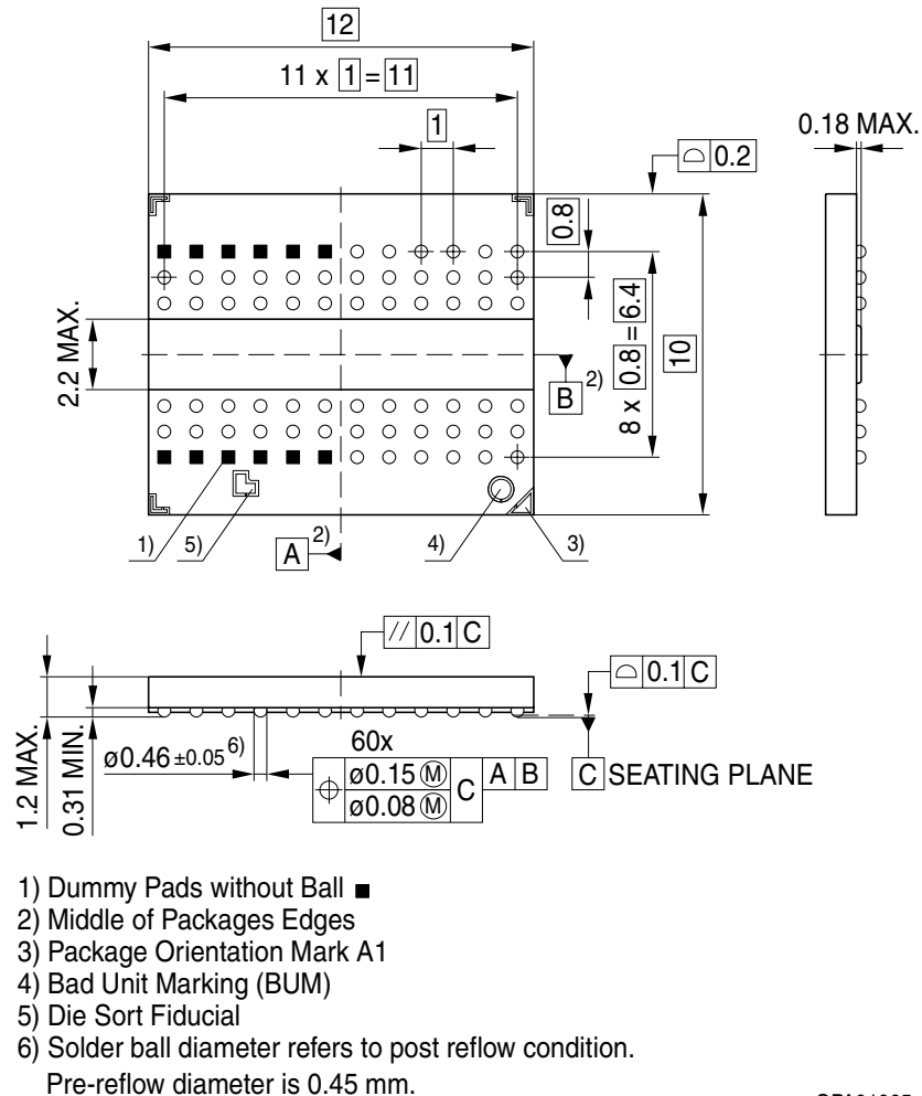
FIGURE 6 Package Outline P(G)-TFBGA-60
