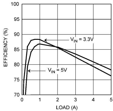
Efficiency V_{OUT} = 0.8V
