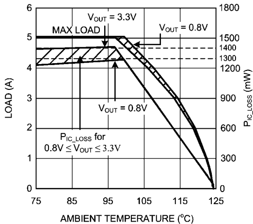
Current Derating V_{IN} = 5V, \theta_{JA} = 20^\circ C / W
