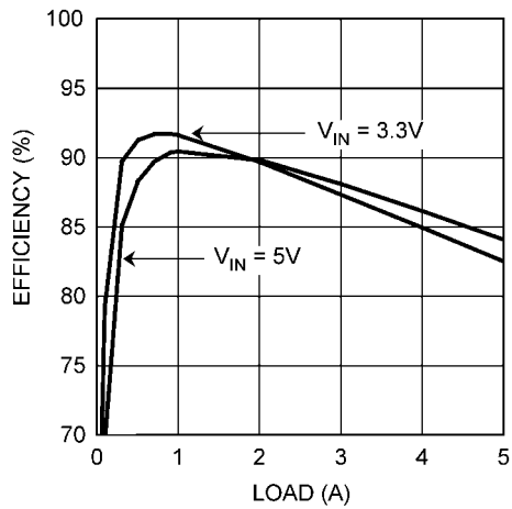
Efficiency V_{OUT} = 1.2V
