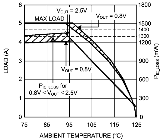
Current Derating V_{IN} = 3.3V, \theta_{JA} = 20^\circ C / W
