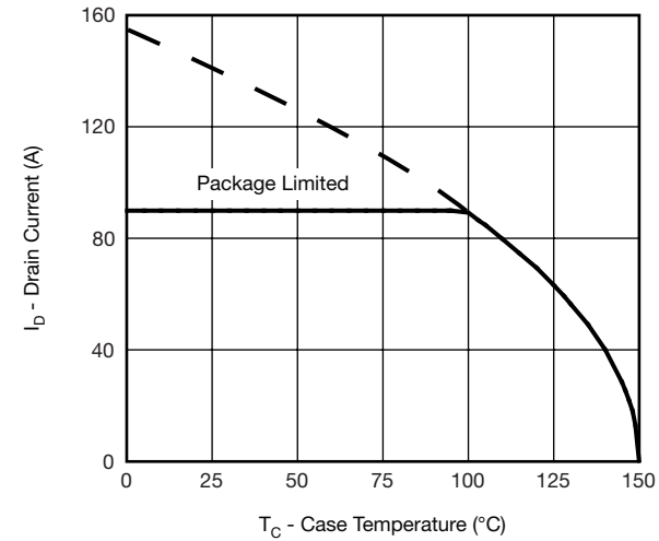
Current Derating
