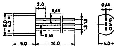
Case Outline 2005A (unit: mm)
