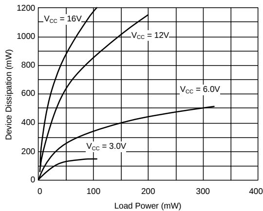
Device Dissipation, 16 \Omega Load
