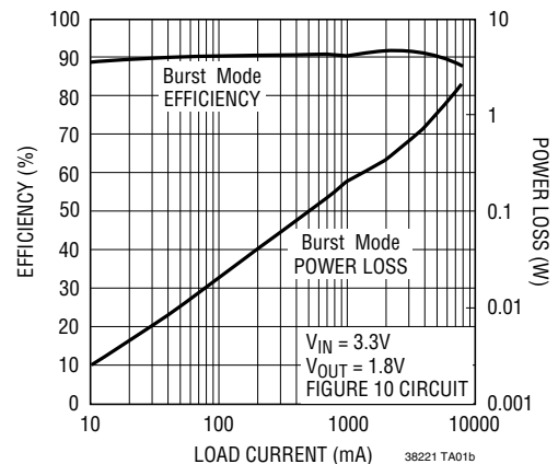
Efficiency/Power Loss vs Load Current
