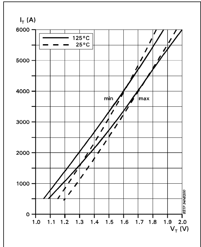
Fig. 3 On-state characteristics.
