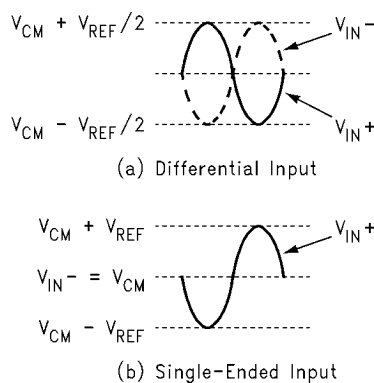
FIGURE 2. Expected Input Signal Range
