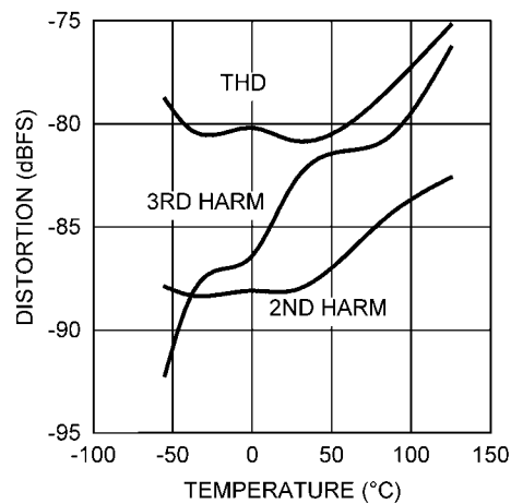
DISTORTION vs. Temperature
