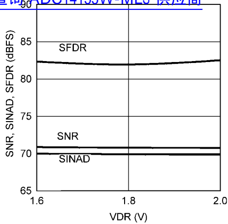
查询"ADC14155W-MLS"供应商 SNR, SINAD, SFDR vs. V_{DR}
