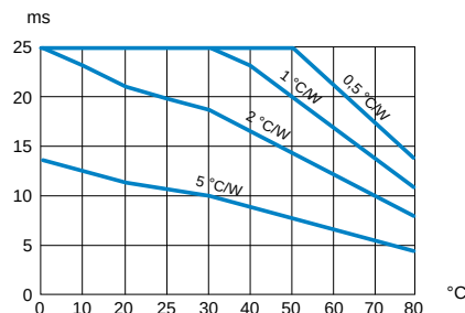
Thermal curves
