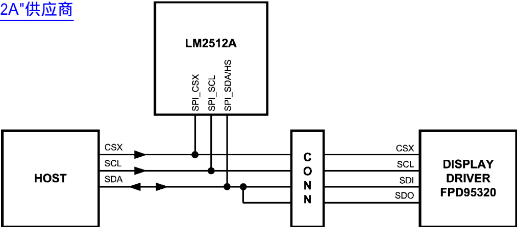
FIGURE 13. LM2512A WRITE & READ to 3-signal SPI HOST
