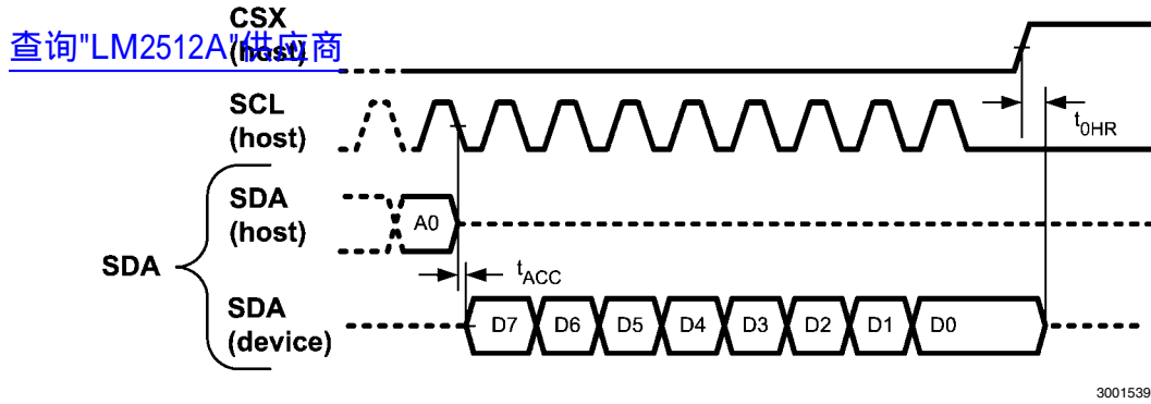
FIGURE 5. SPI Interface
