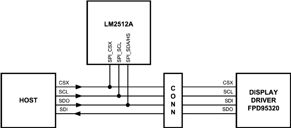
FIGURE 14. LM2512A WRITE only to 4-signal SPI HOST
