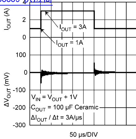
Load Transient Response, C_{OUT} = 100\ \mu\text{F} Ceramic 查询"LP38859"供应商
