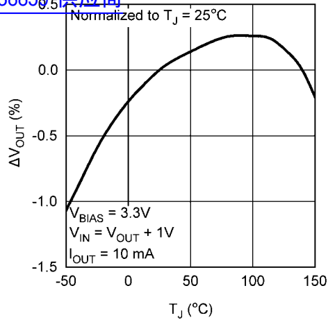
V_{OUT} vs Temperature 查询"LP38859"供应商
