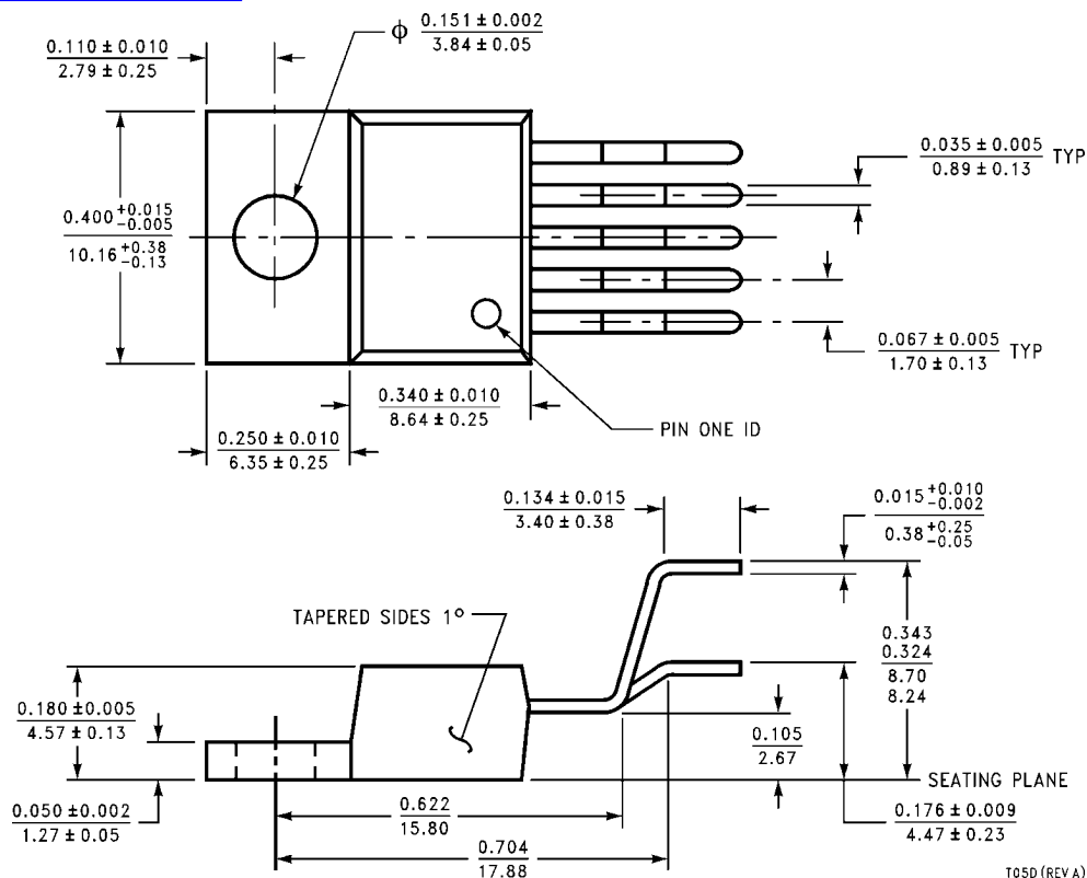
TO-220 5-Lead, Stagger Bend Package (TO220-5) NS Package Number TO5D
