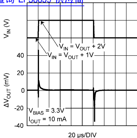
V IN Line Transient Response 查询"LP38859"供应商
