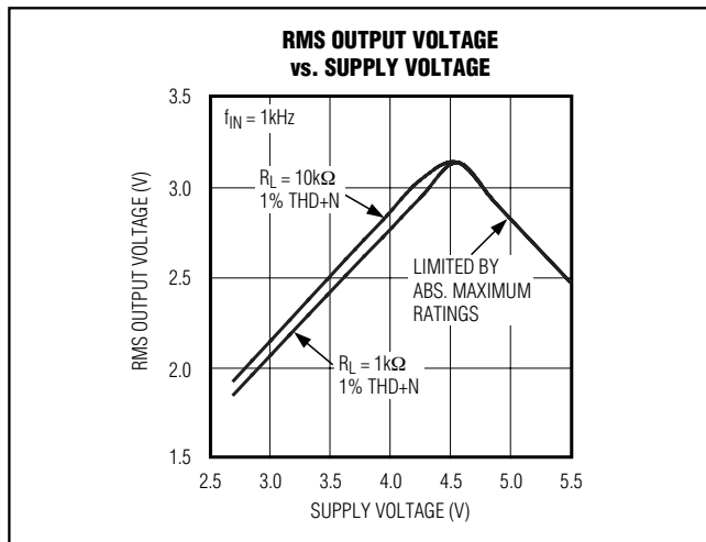
Figure 4. RMS Output Voltage vs. Supply Voltage
